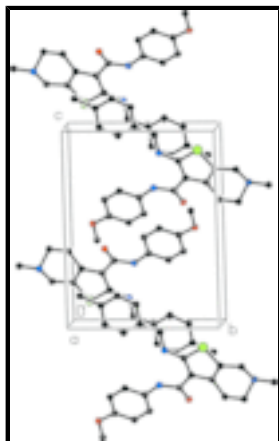
Fig. 2. Packing diagram of (I); all H-atoms are omitted for clarity.
