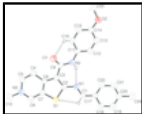
Fig. 1. The molecular structure of the title compound, showing the atom-labeling scheme with displacement ellipsoids drawn at the 50% probability level. Dashed lines indicates intramolecular H-bonds.
